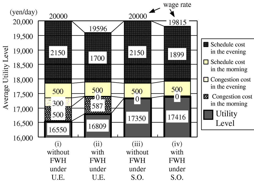
Figure 9. Average Values of Cost Items with / without FWH ( \alpha = 0.2 )
