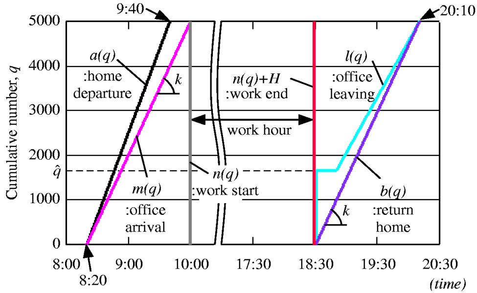
Figure 1. Non-Flexible Pattern under User Equilibrium
