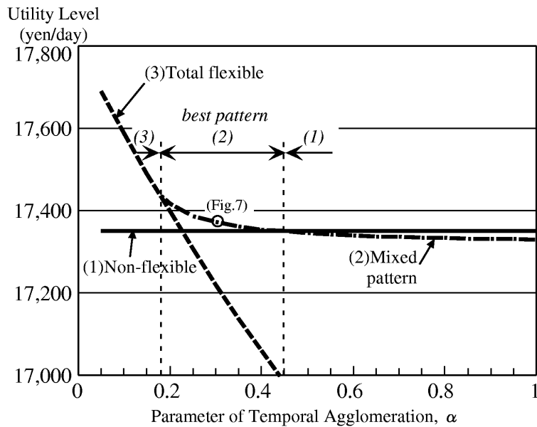
Figure 8. Utility Levels of the Three Patterns under System Optimum
