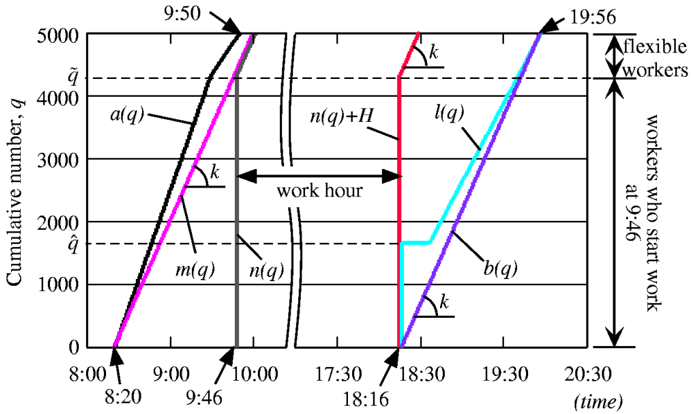
Figure 2. Mixed Pattern 1 under User Equilibrium ( \alpha = 0.8 )
