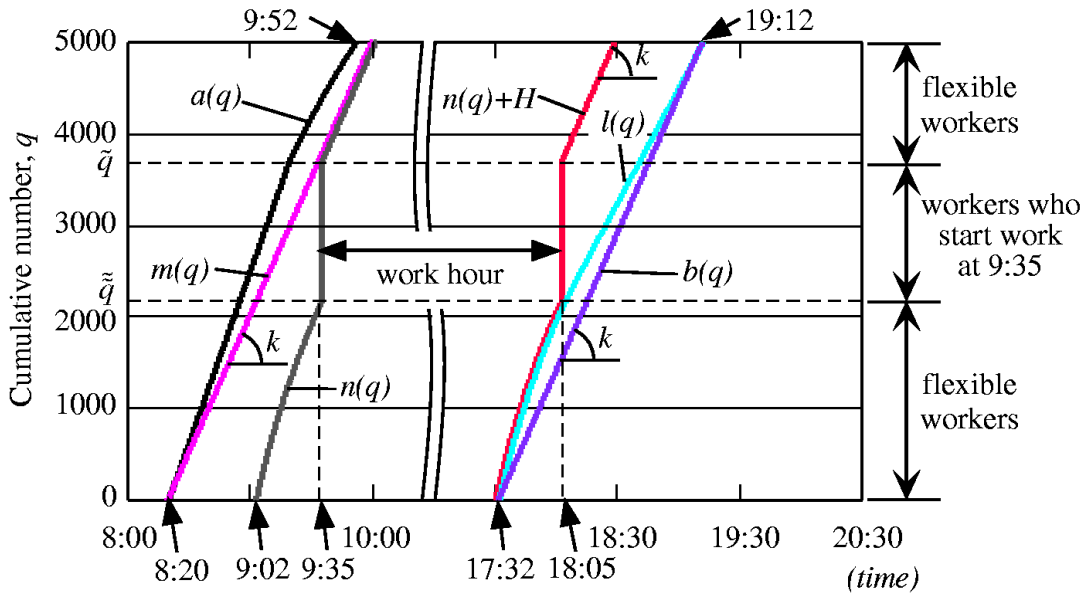
Figure 4. Mixed Pattern 3 under User Equilibrium ( \alpha = 0.4 )
