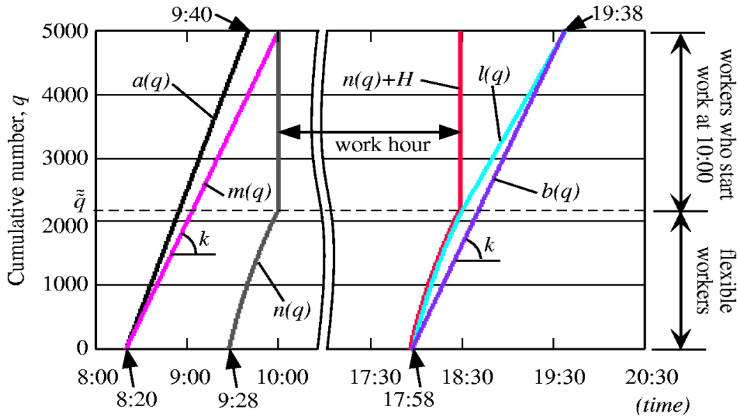
Figure 3. Mixed Pattern 2 under User Equilibrium ( \alpha = 0.4 )
